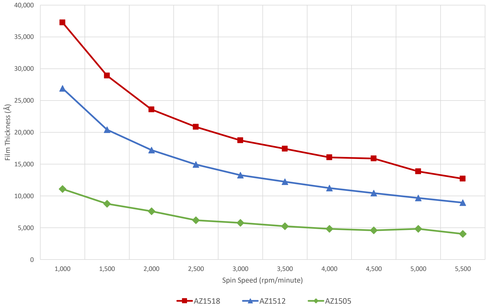
Spin speed vs Film Thickness
