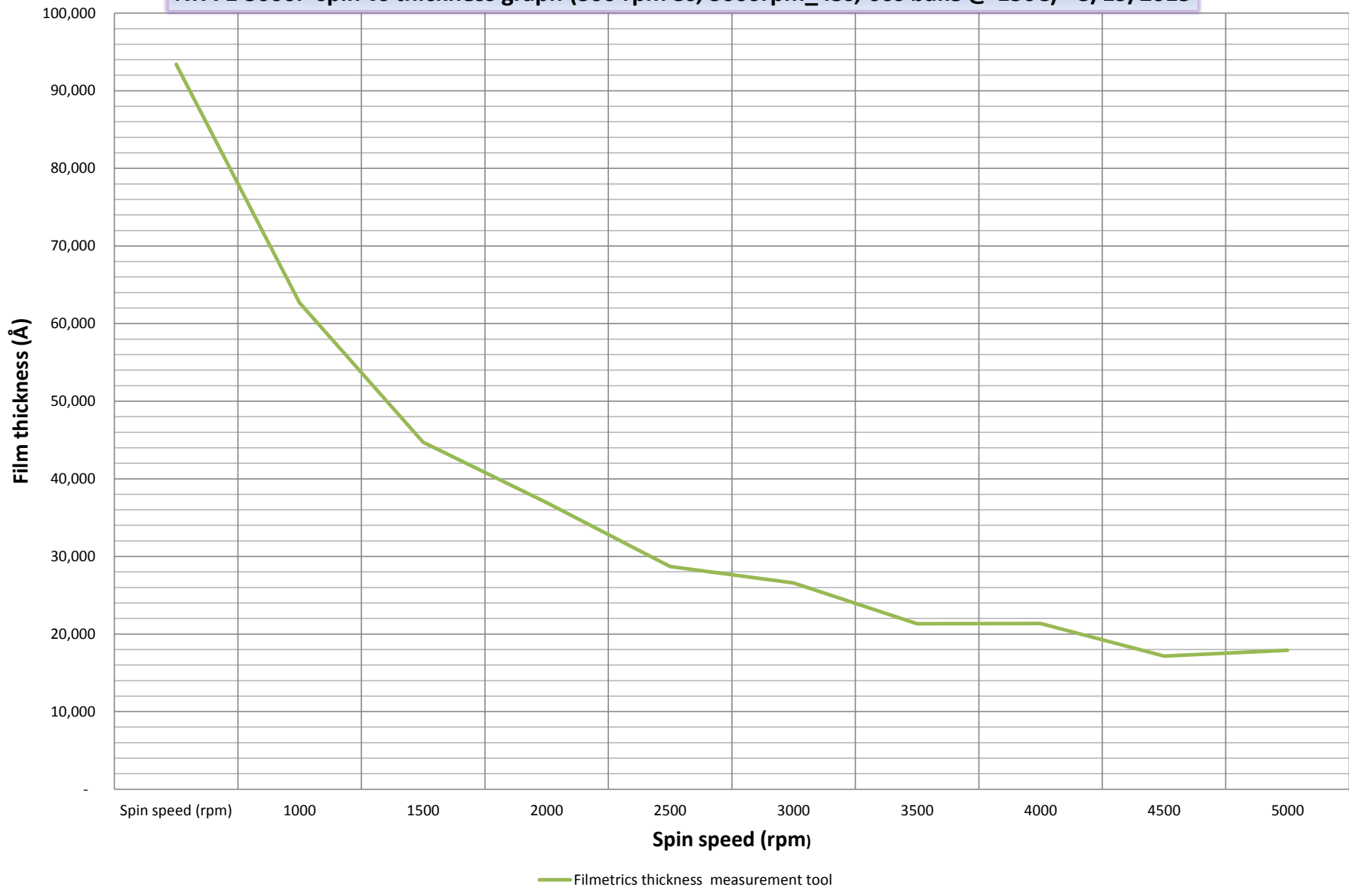
NR 71 3000P spin vs thickness graph (300 rpm 3s, 3000rpm_45s, 60s bake @ 150C) - 5/19/2015
