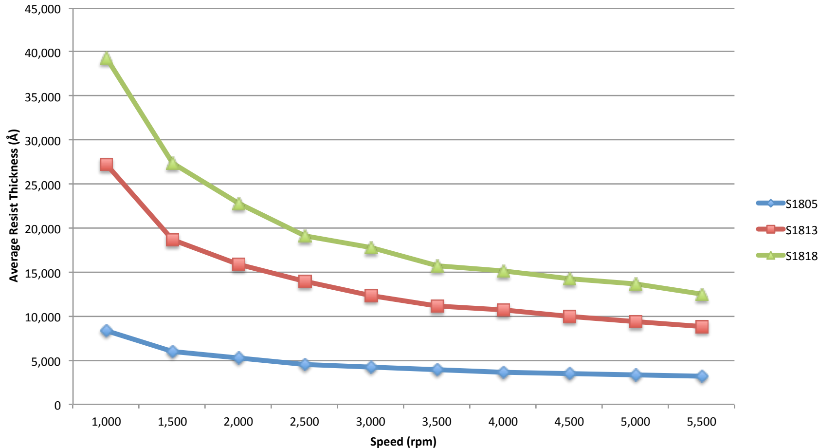
S1800 Series Resist Average Thickness vs. Speed
